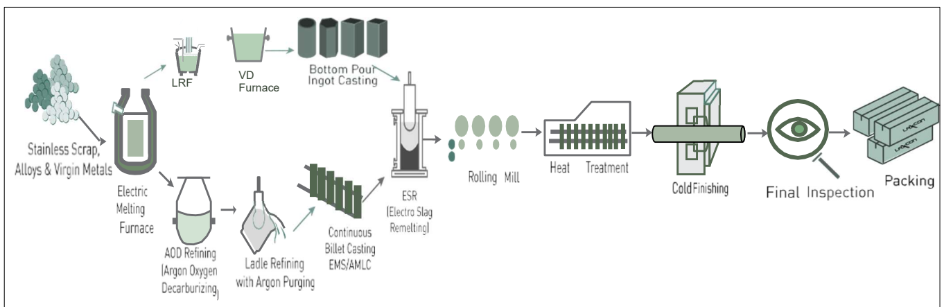
Figure 1 Product making Process for Stainless Steel Cast & Rolled Products at Laxcon Steels
